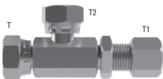
Female Straight X Bulkhead Tube Fitting X Female Straight
