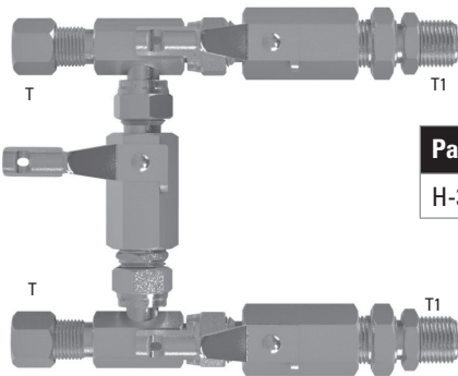
Tube Fitting x Male Straight Reverse Bulkhead
